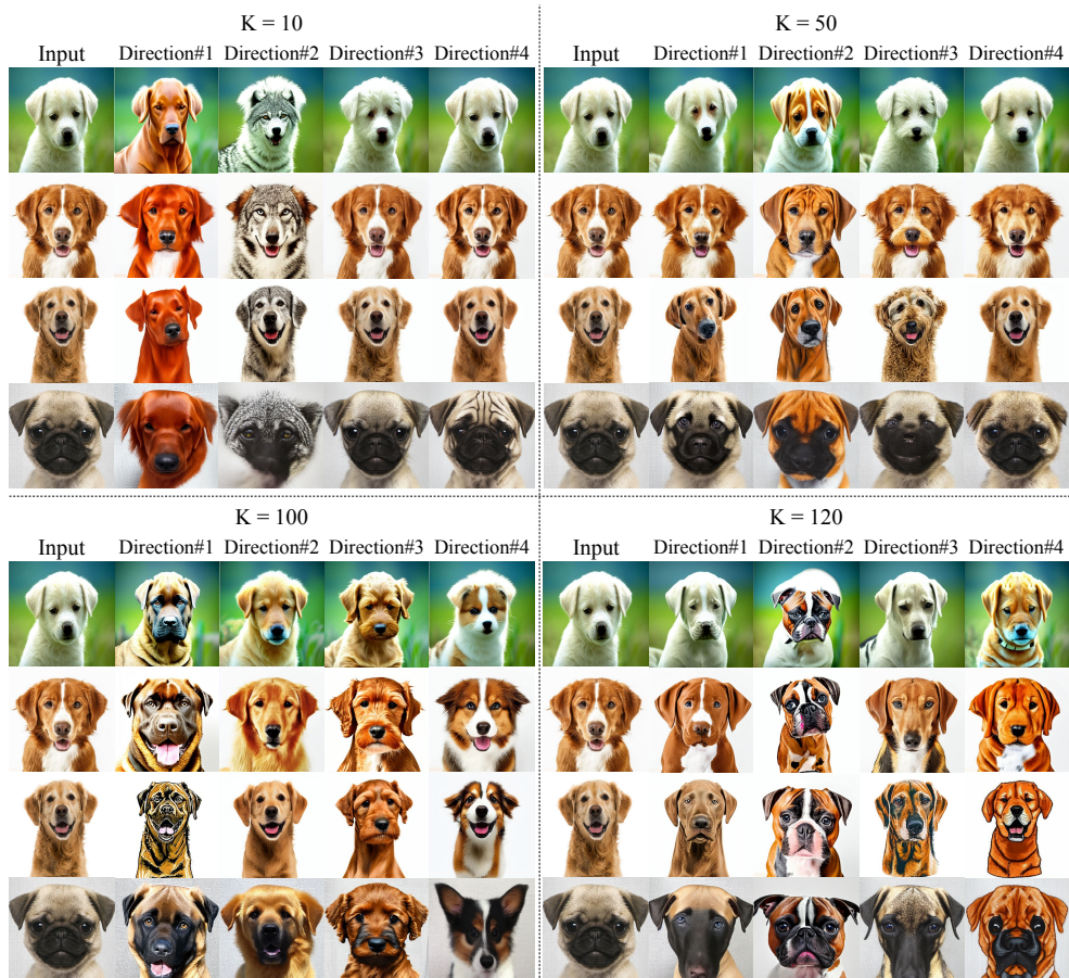
Figure S.4: Ablation study of K . We show transformation results with varying K values (10, 50, 100, 120). The number of learned directions K directly impacts the quality of transformations.
